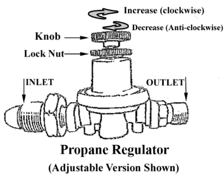
Propane Regulator
